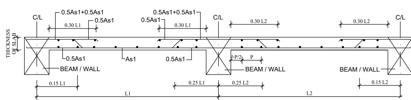
TYPICAL SECTION THROUGH SLAB
