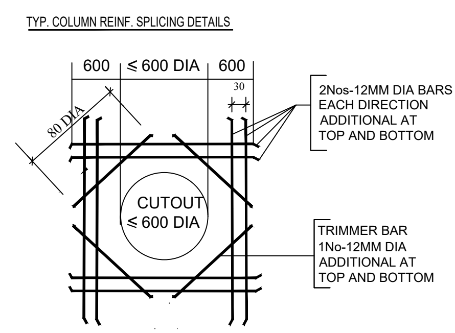
ADDITIONAL REINFORCEMENT AROUND CIRCULAR CUT-OUT (OPENING) IN SLAB
