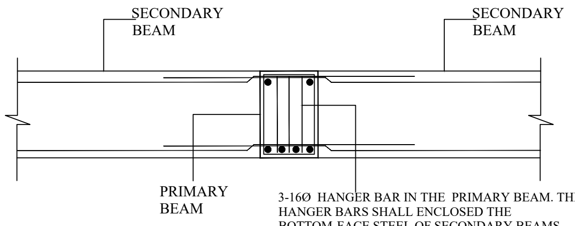
TYPICAL JUNCTION DETAILS OF MAIN & SECONDARY BEAMS
