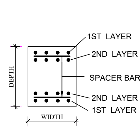
TYP. SEC. OF MAIN BEAM (STIRRUPS NOT SHOWN)
