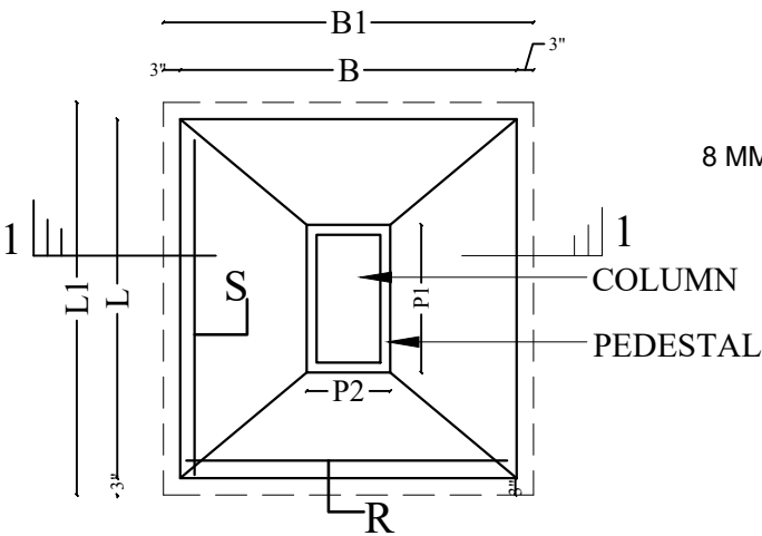
TYPICAL PLAN OF COLUMN FOOTING
